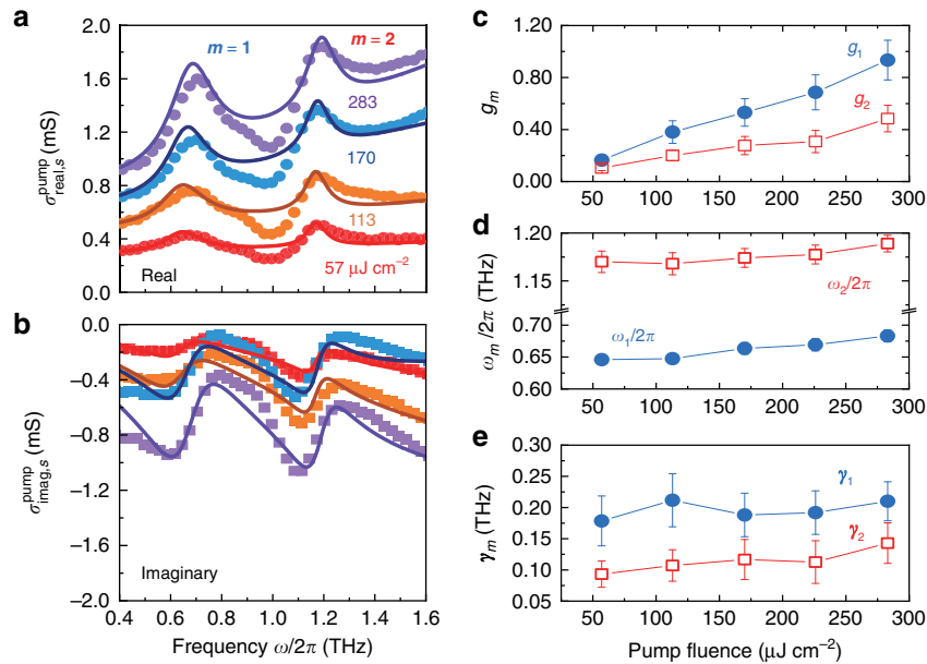
Fig. 3 Pump fluence-dependent THz photoconductivity spectra for MAPbI 3 polycrystalline grains. Extracted a real and b imaginary parts of THz photoconductivity spectra of MAPbI 3 polycrystalline grains, following photoexcitation at 1.55 eV with pump fluences of 57, 113, 170, and 283 \mu\text{J cm}^{-2} at 300 K. The solid lines are the DSL model fits. Pump fluence evolutions of c oscillator strength g_m , d resonant frequency \omega_m/2\pi , and e FWHM linewidth \gamma_m of the resonance modes
