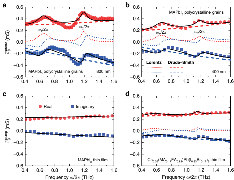
Fig. 2 The observation of photoinduced large polaron in MAPbI 3 . Real (circles) and imaginary (squares) parts of the sheet photoconductivity spectra of MAPbI 3 polycrystalline grains for two different pumped energies of a 1.55 eV and b 3.1 eV, at \Delta t = 5 ps. The complex sheet photoconductivity spectra for c MAPbI 3 thin film and d Cs 0.05 (MA 0.17 FA 0.83 )Pb(I 0.83 Br 0.17 ) 3 thin film with pumped energy of 3.1 eV, at \Delta t = 5 ps. The black curves in (a) , (b) , and (d) represent the Drude-Smith-Lorentz fits. The dashed and dotted lines show the components for the Drude-Smith term and the Lorentz terms, respectively
